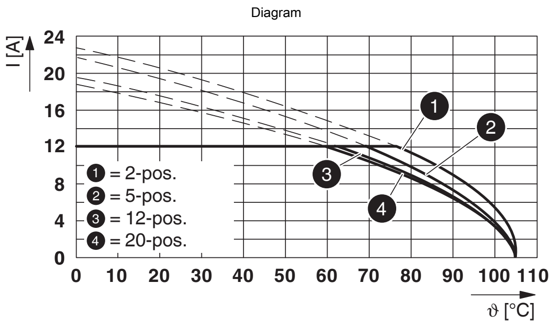
Type: FKCT 2,5/...-ST-5,08 with MSTBA 2,5/...-G-5,08
