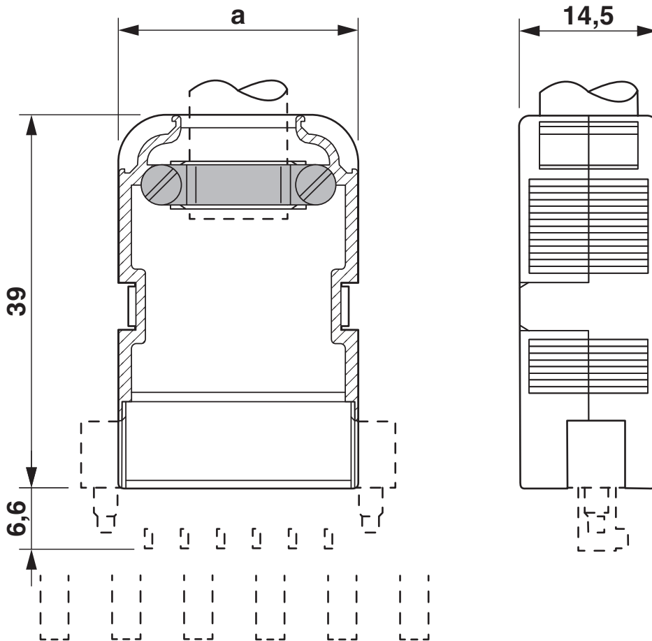
Dimensional drawing
