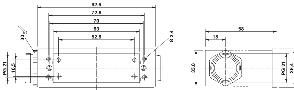
Dimensional drawing
