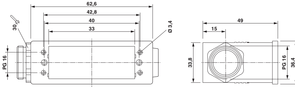
Dimensional drawing
