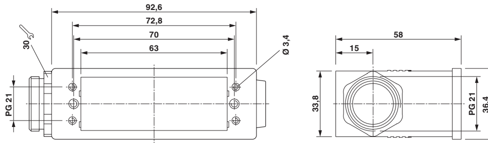
Dimensional drawing
