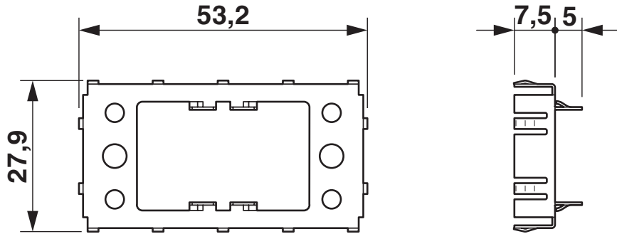
Dimensional drawing
