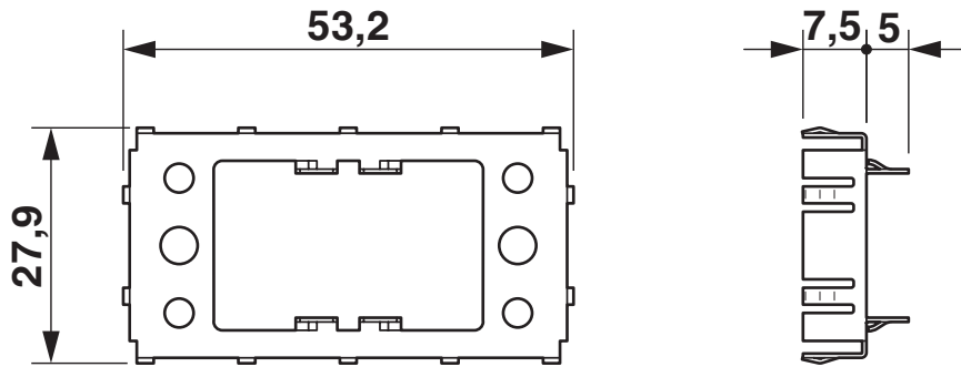
Dimensional drawing
