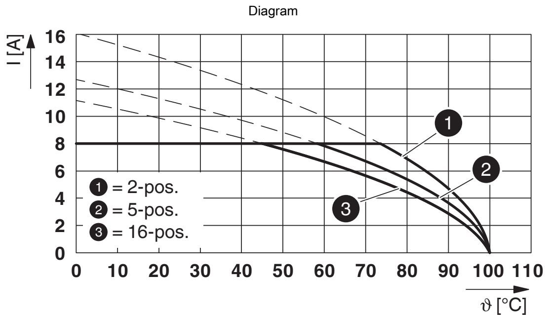
Type: MCV(W/R) 1,5/10-STF-3,81 with MCV 1,5/10-GF-3,81
