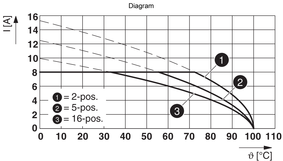
Type: MCV(W/R) 1,5/10-STF-3,81 with MCD 1,5/10-G1F-3,81
