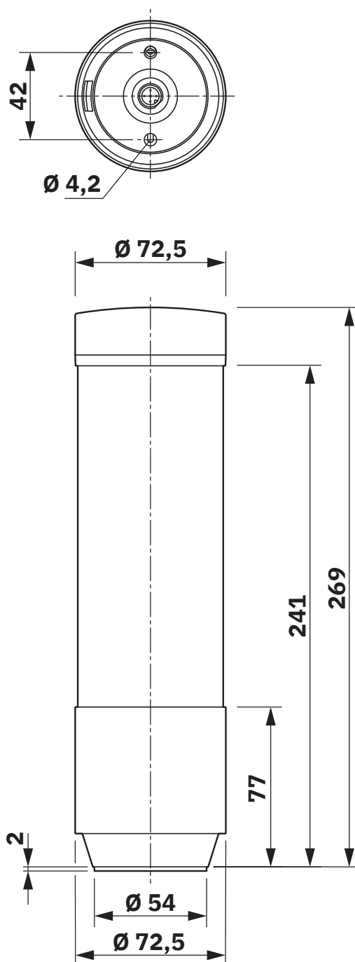
Dimensional drawing
