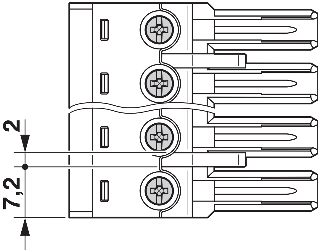
Dimensional drawing
