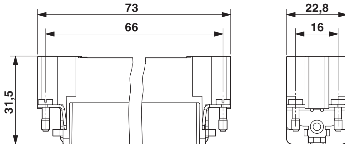
Male insert (turned contacts)
