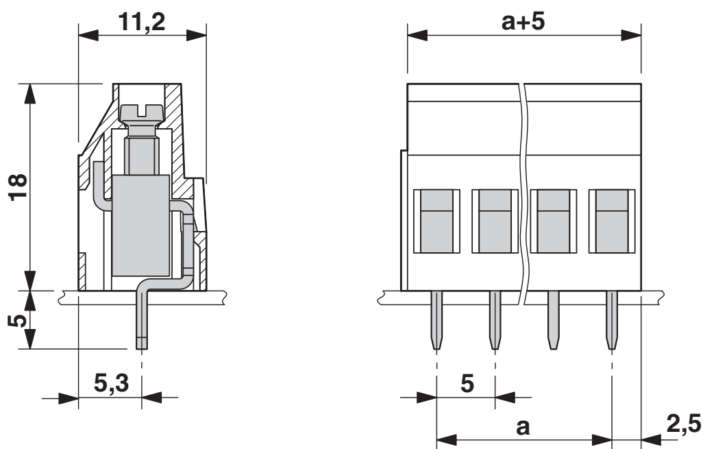
Dimensional drawing
