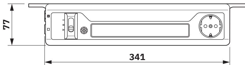
Schematic diagram
