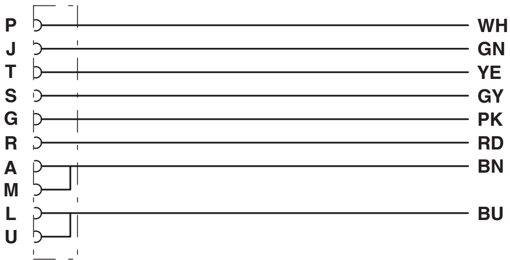
Contact assignment of the M16 socket
