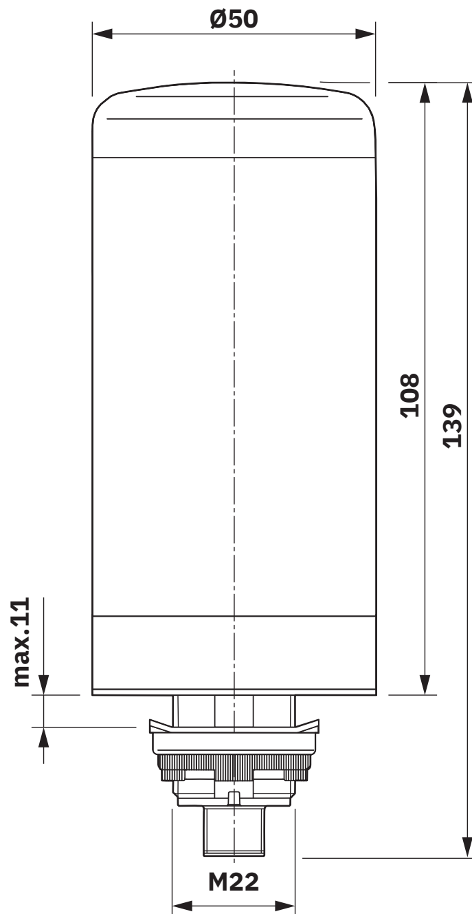
Dimensional drawing
