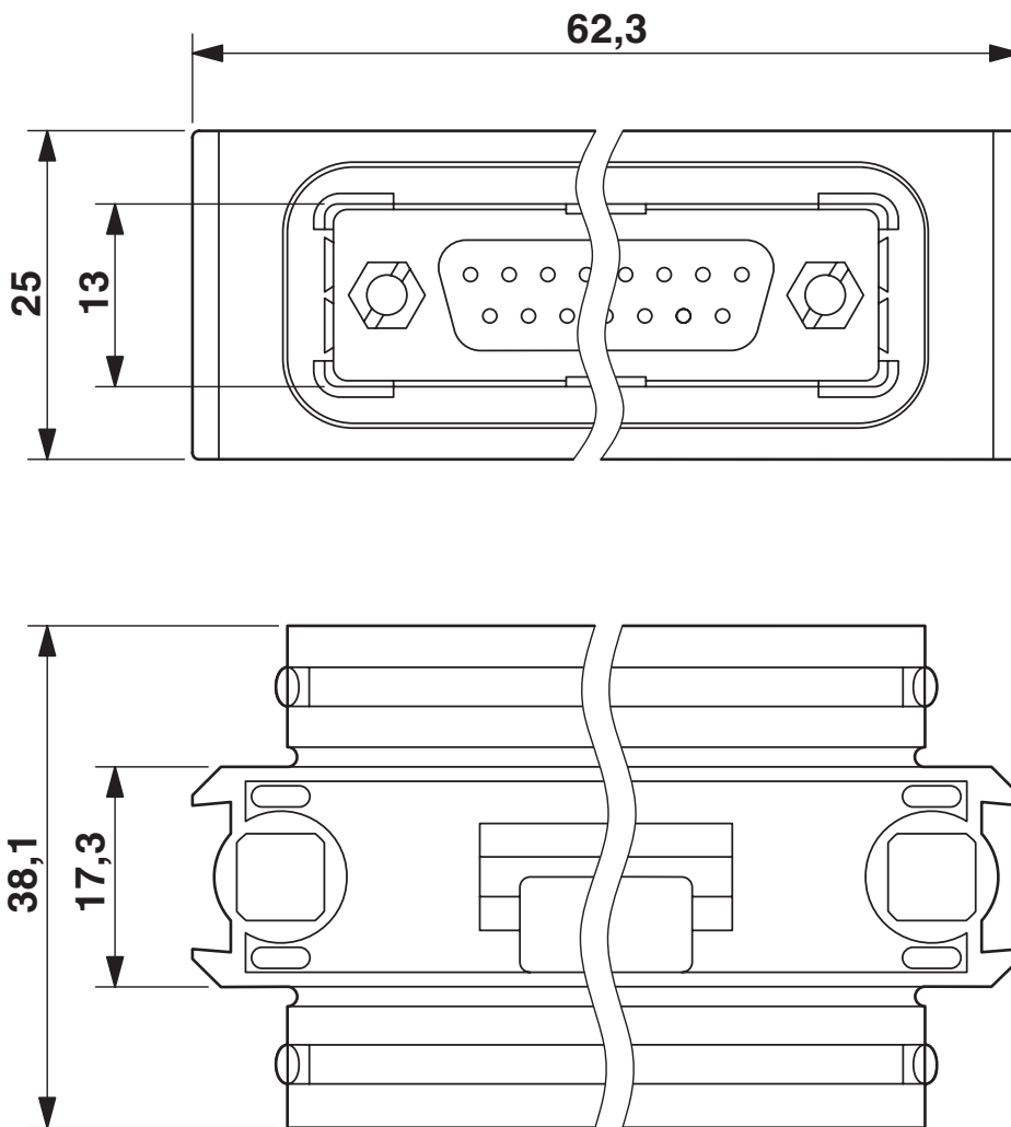
Dimensional drawing
