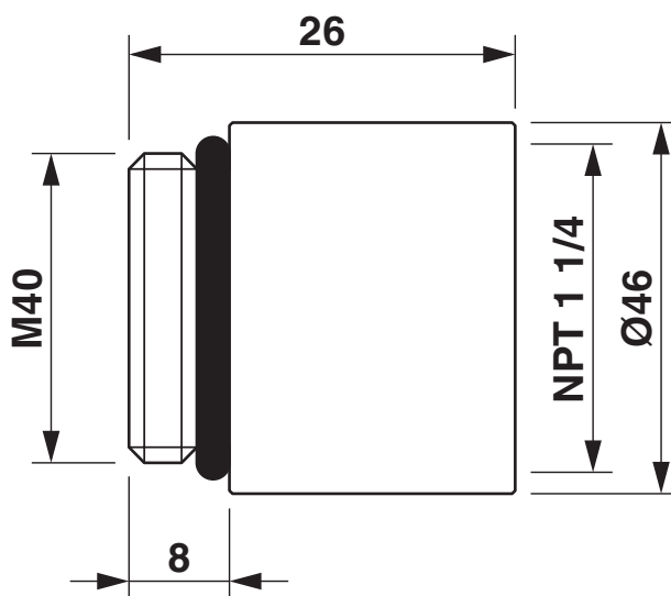
Dimensional drawing
