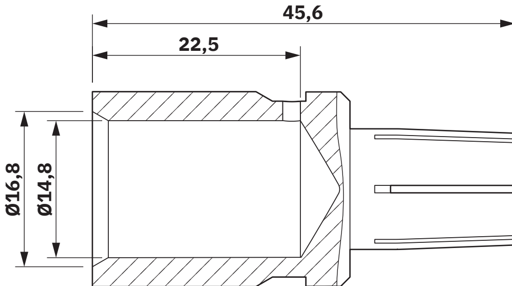
Dimensional drawing
