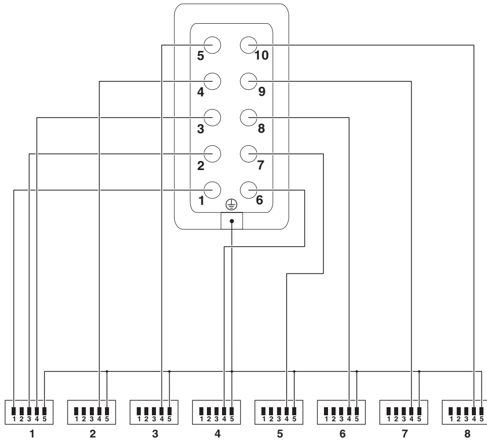
Circuit diagram
