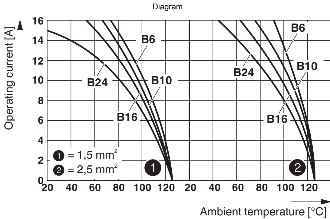
Derating diagram HC-B10-EBUC
