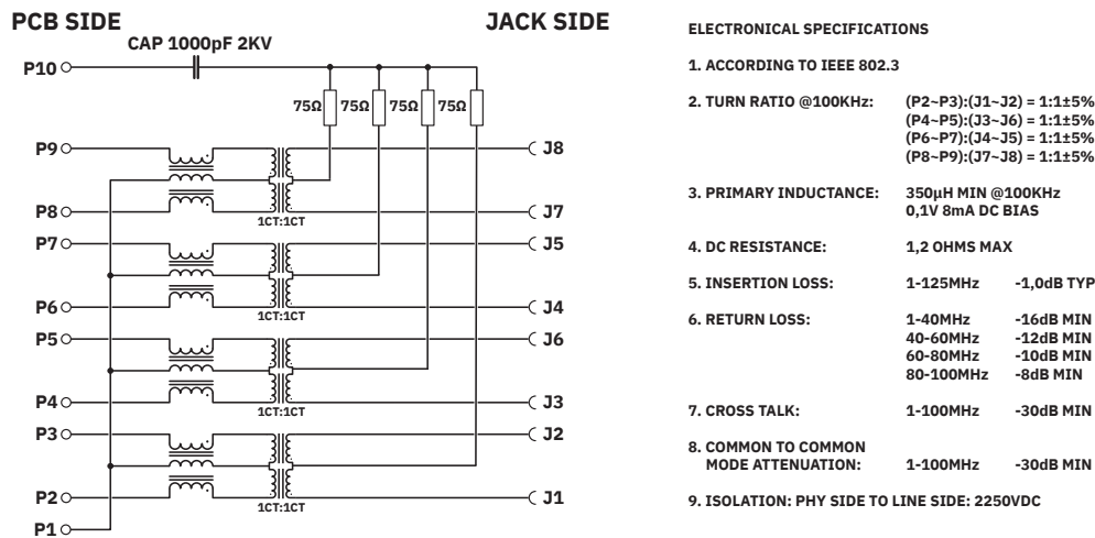
Circuit diagram
