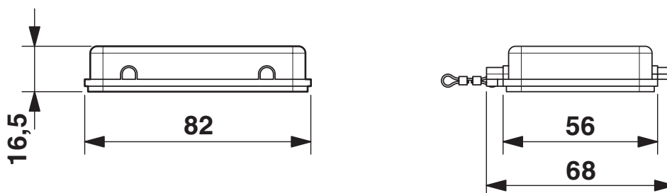
Dimensional drawing
