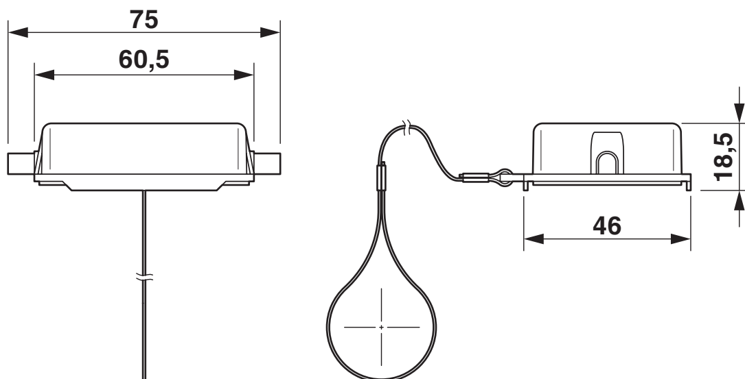
Dimensional drawing
