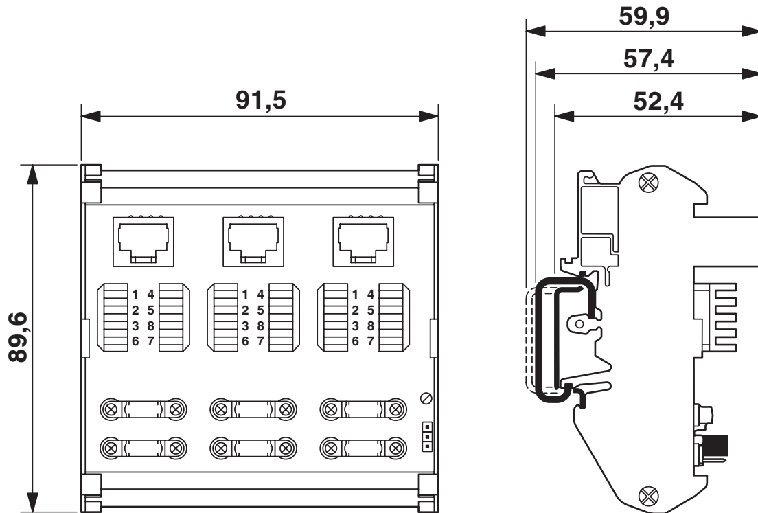
Patch panel with three RJ45 connections
