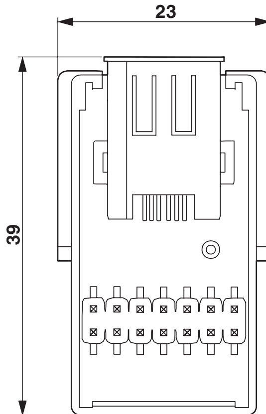
Dimensional drawing
