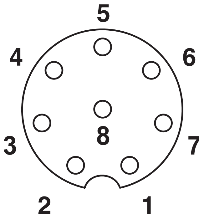
Pin assignment of M12 push-pull female, 8-pos., A-coded, view of female side
