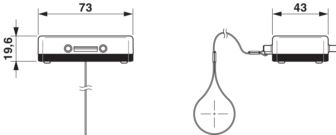
Dimensional drawing
