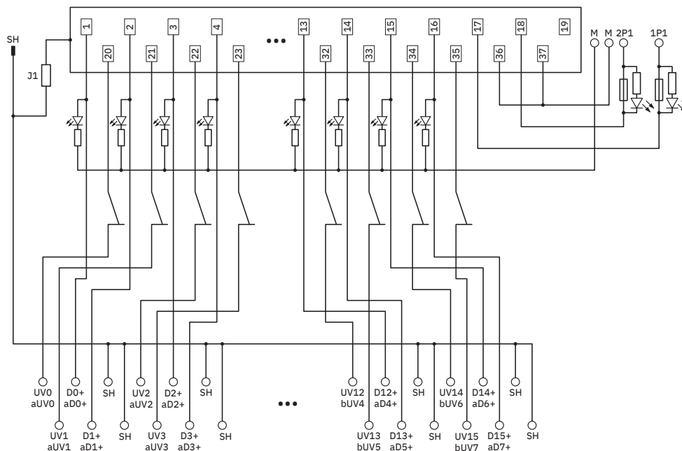
Circuit diagram
