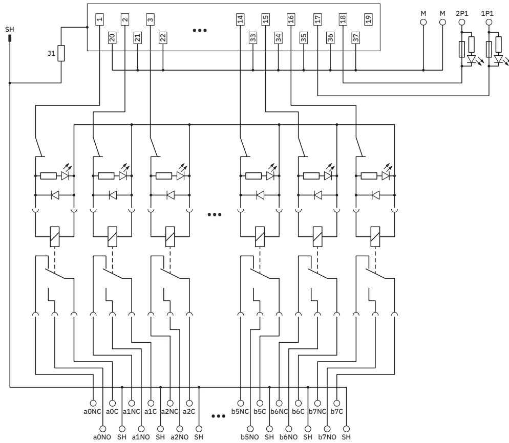
Circuit diagram
