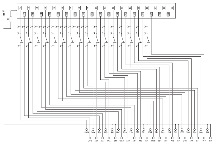
Circuit diagram
