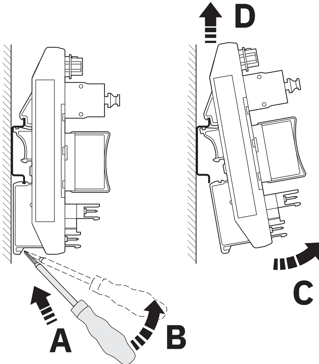
Schematic diagram
