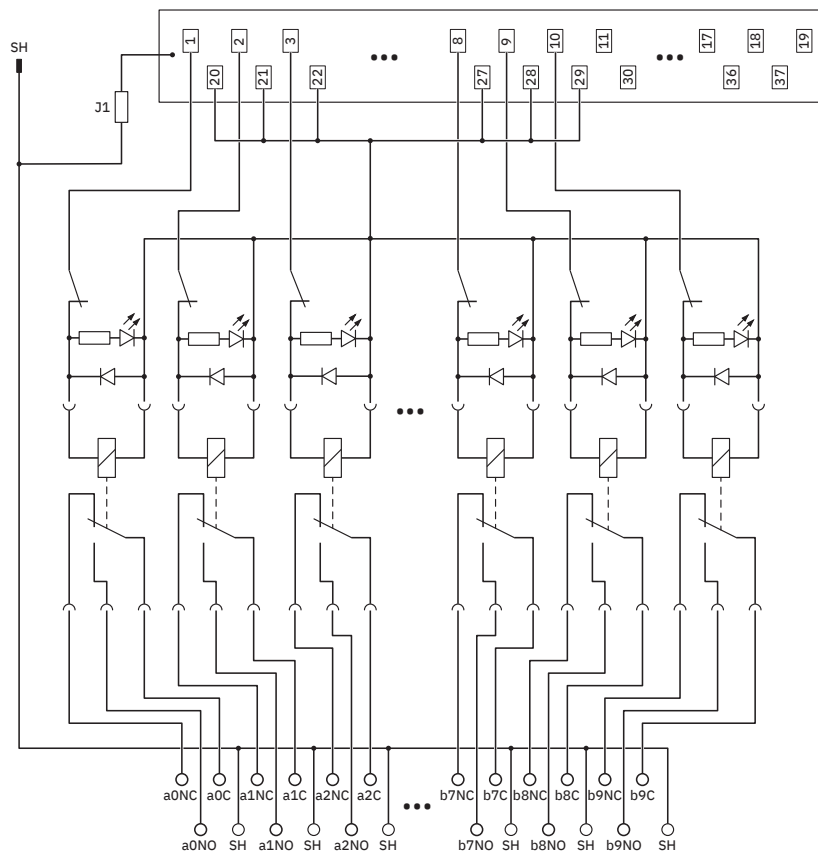
Circuit diagram
