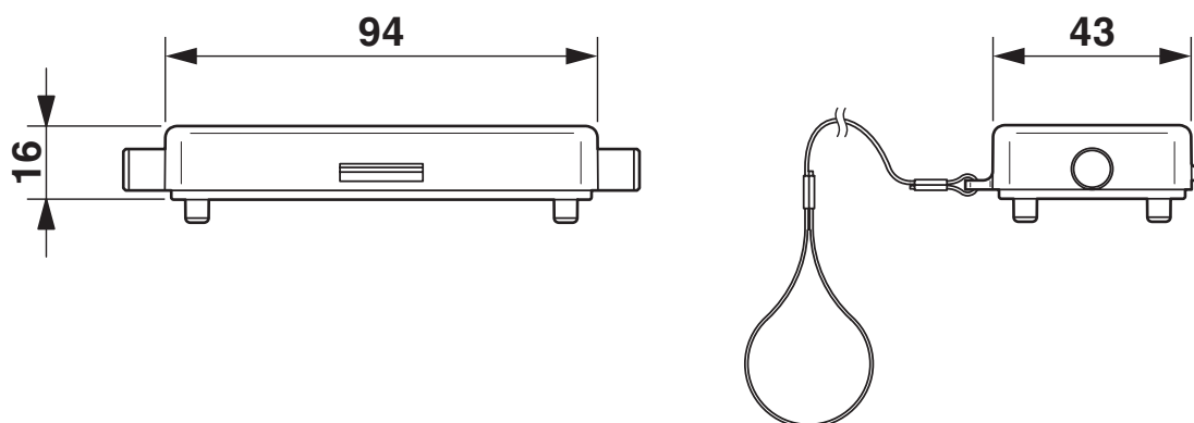
Dimensional drawing
