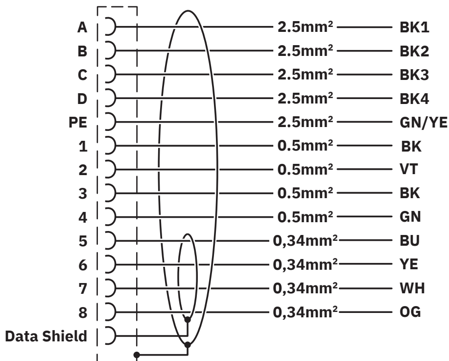
Circuit diagram
