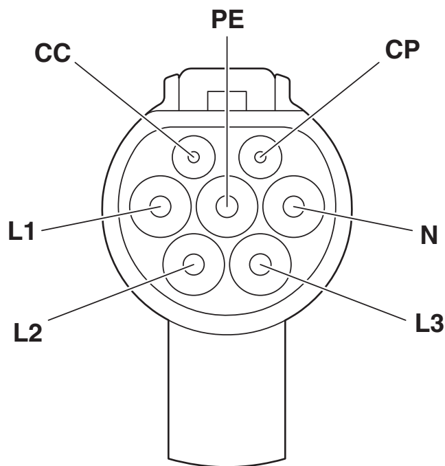
Connection diagram
