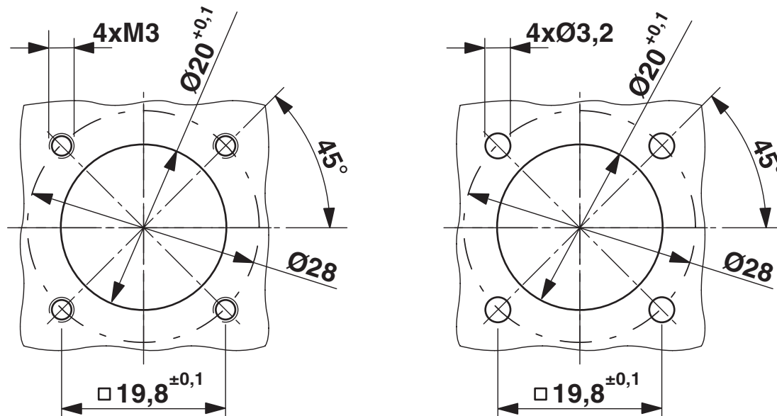
Installation dimensions
