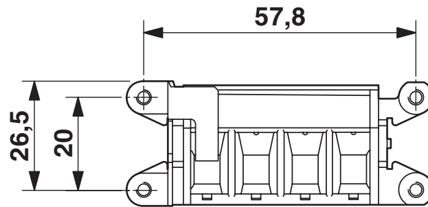
Dimensional drawing
