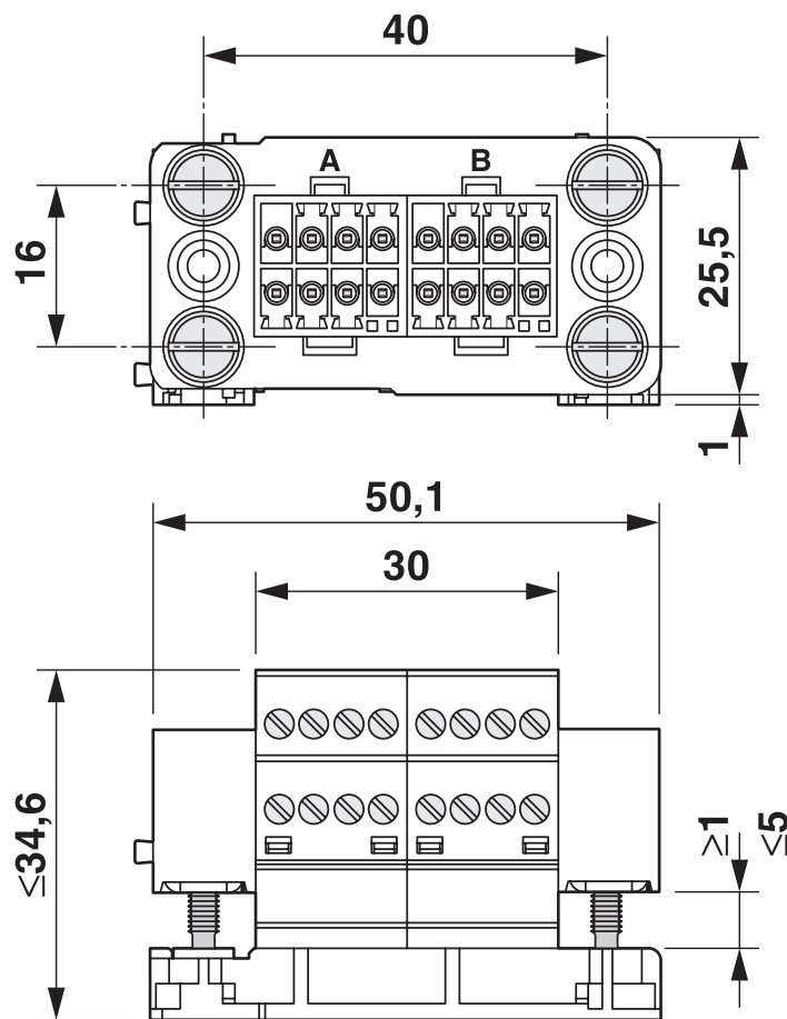
Dimensional drawing
