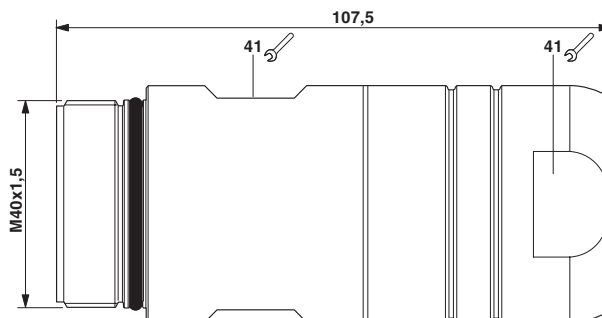
Dimensional drawing
