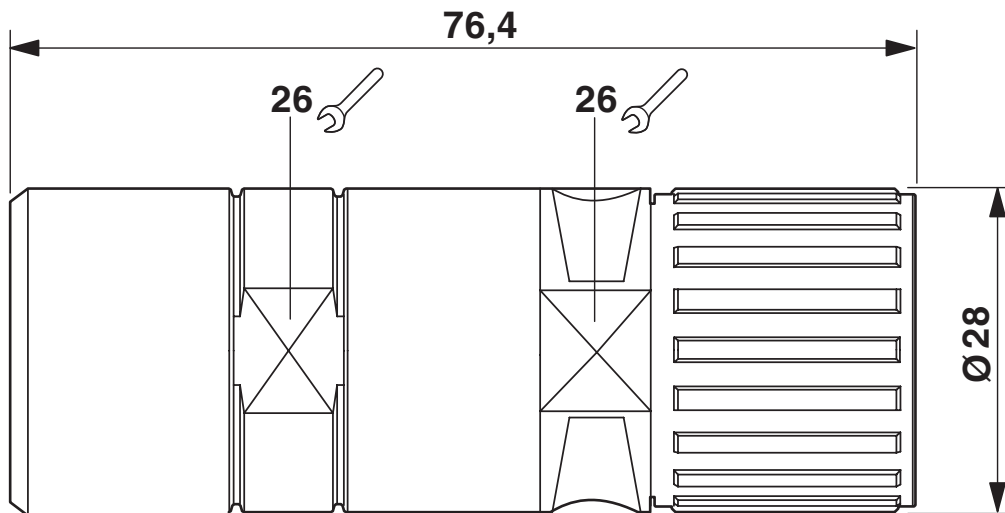
Dimensional drawing
