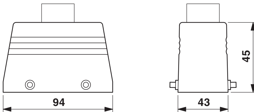
Dimensional drawing
