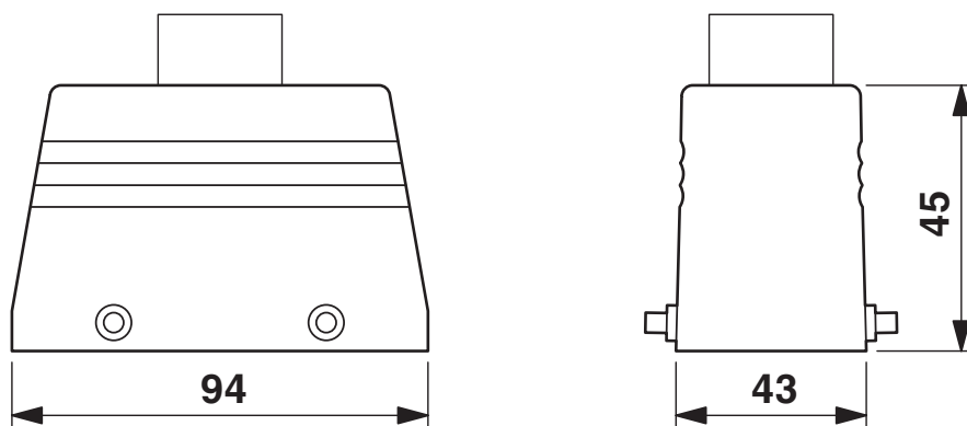
Dimensional drawing
