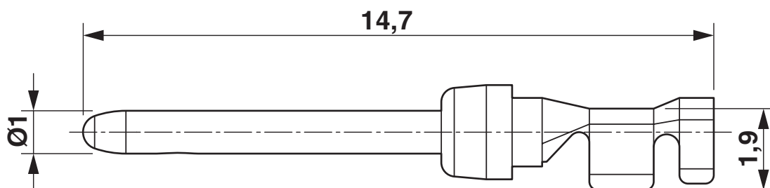
Dimensional drawing
