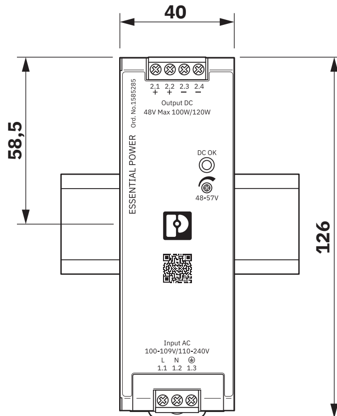
Dimensional drawing
