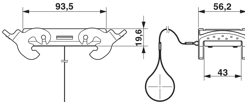
Dimensional drawing
