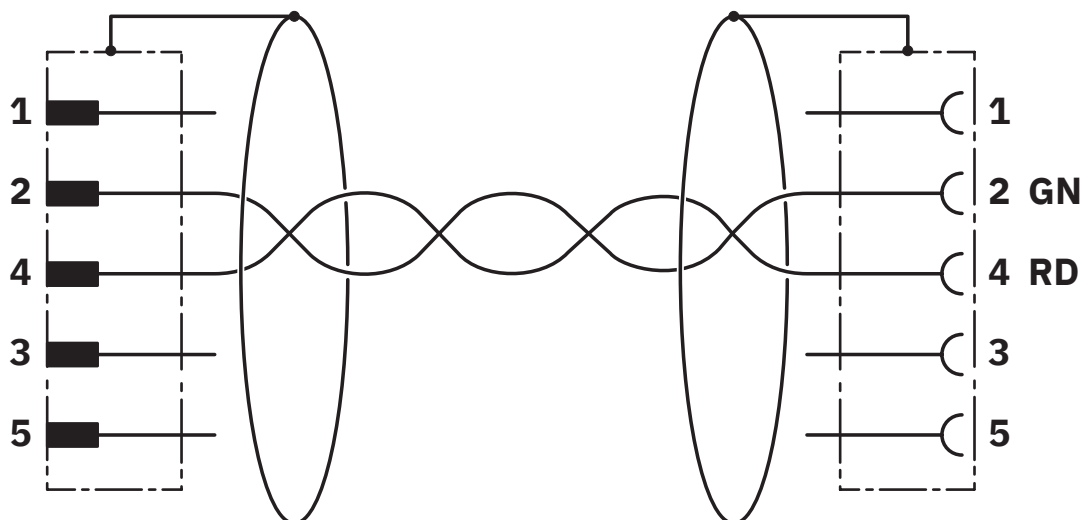
Circuit diagram
