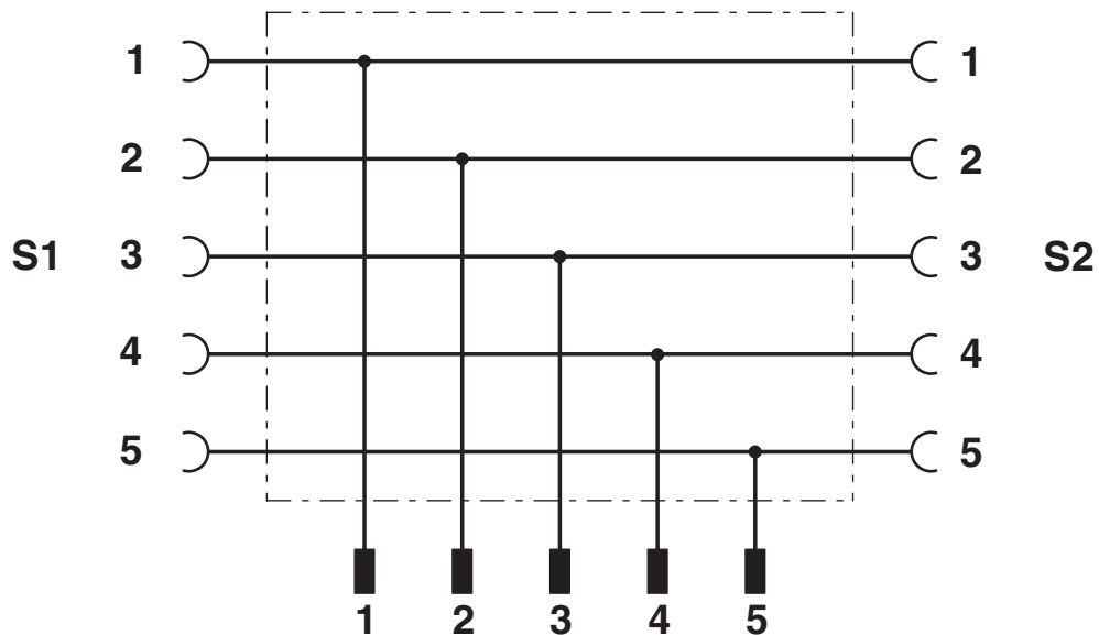
Contact assignment of the M12 Y distributor
