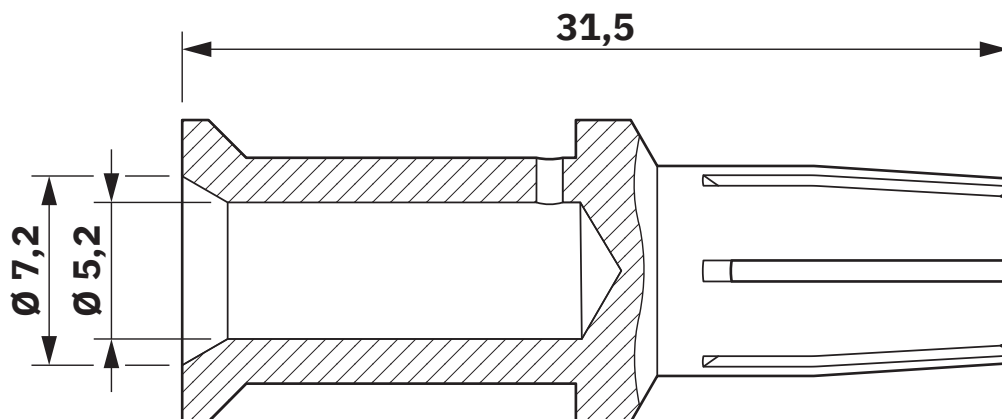
Dimensional drawing
