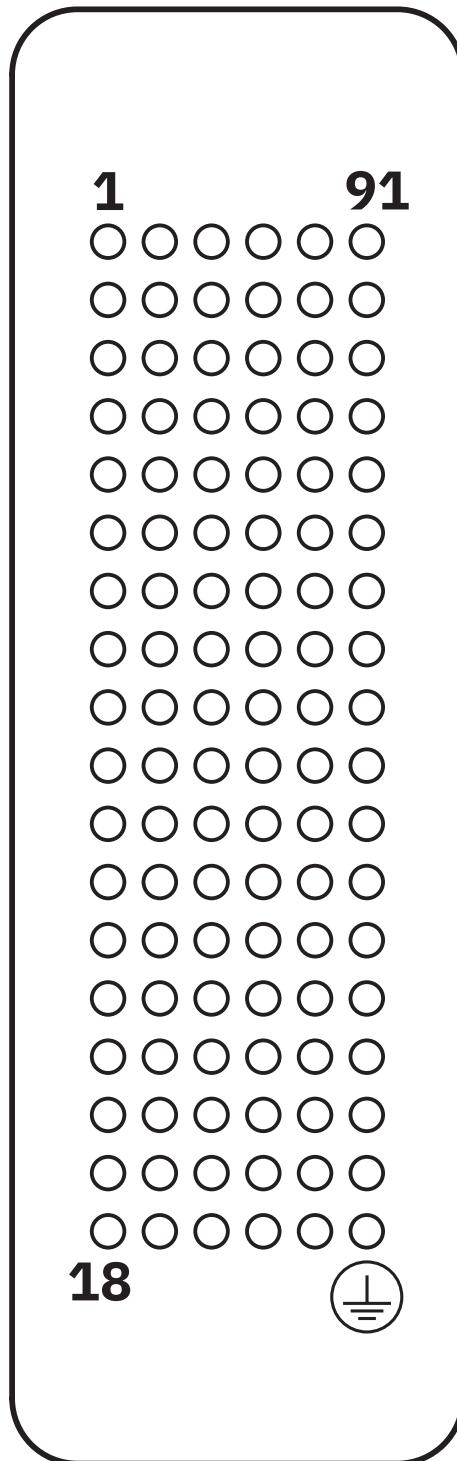
Schematic diagram
