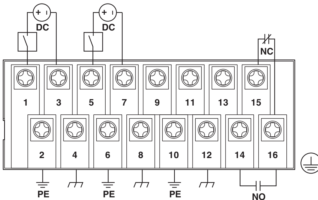
Connection diagram
