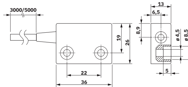
Dimensional drawing
