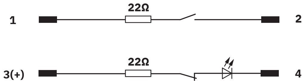
Circuit diagram
