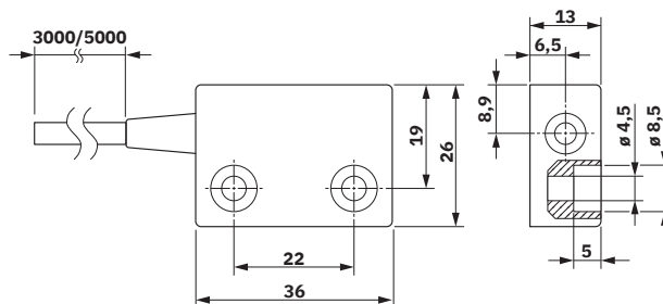
Dimensional drawing
