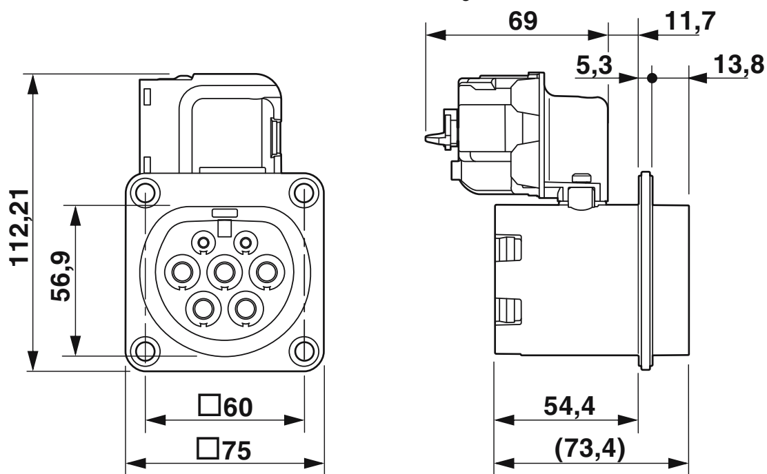
Dimensional drawing
